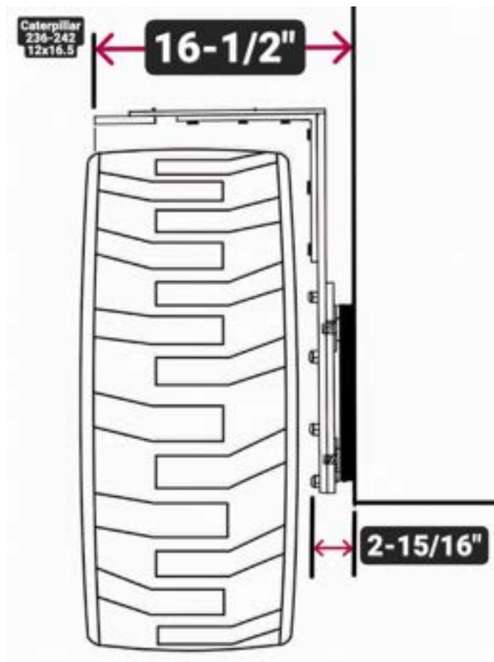
Figure 3B: Inside Dimension
